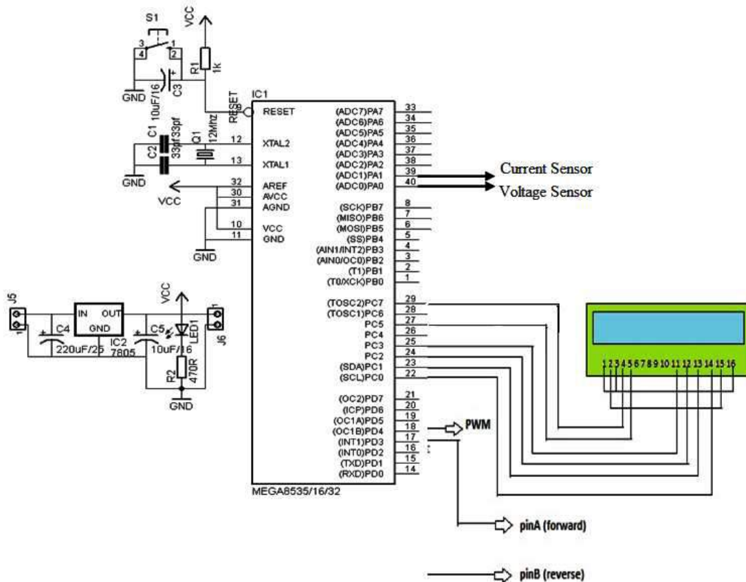
FIGURE 4. Minimum system requirement for microcontroller ATmega8535
