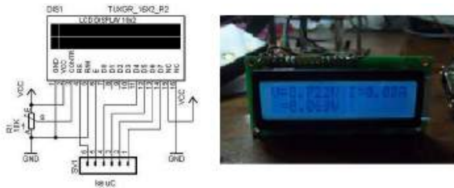
FIGURE 6. The schematic view of LCD 2×16 byte
