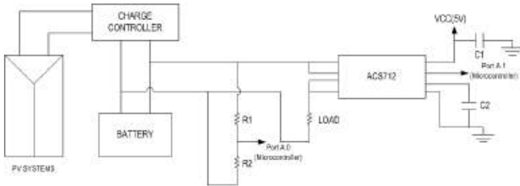
FIGURE 1. The schematic diagram of real-time output power visualization of PV systems
